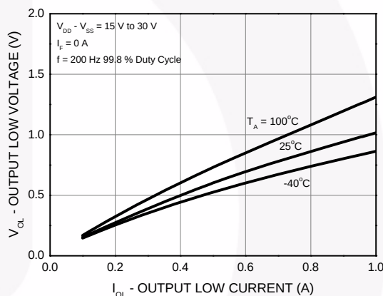
Figure 7. Output Low Voltage vs. Output Low Current
