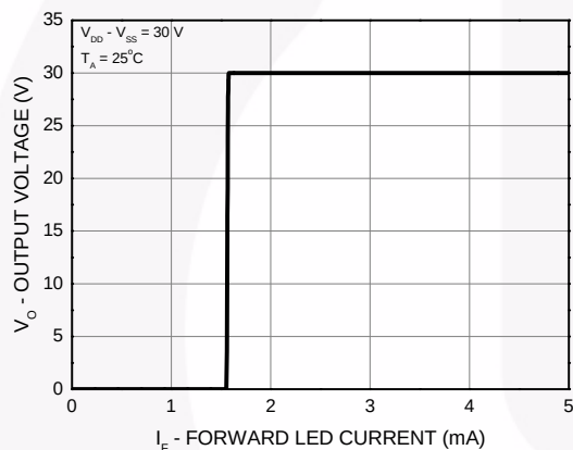
Figure 18. Transfer Characteristics
