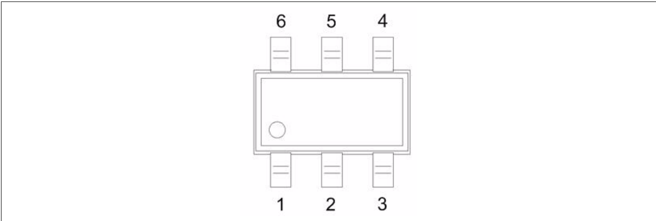
Figure 2 TLE493D-W2B6 pinout
