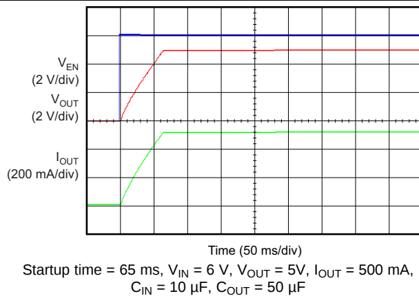
Figure 21. Startup
