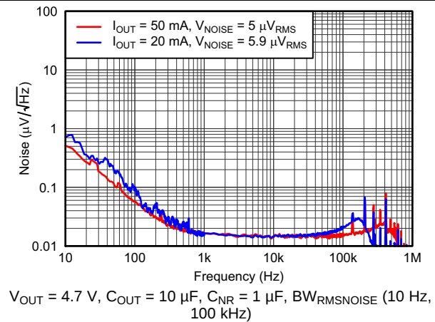
Figure 22. Noise vs Output Current
