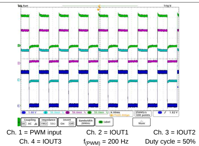
Figure 10. PWM Dimming
