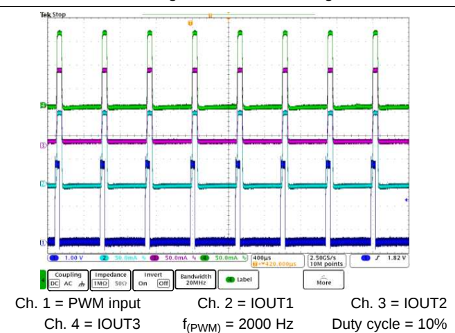
Figure 12. PWM Dimming
