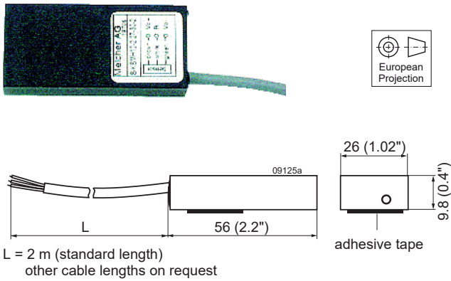
Fig. 26 Temperature sensor
