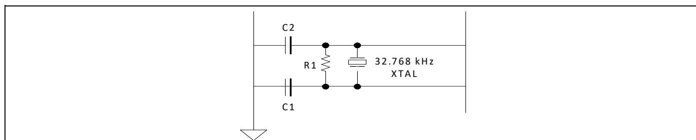
Figure 3 Recommended 32 kHz oscillator electrical specification
