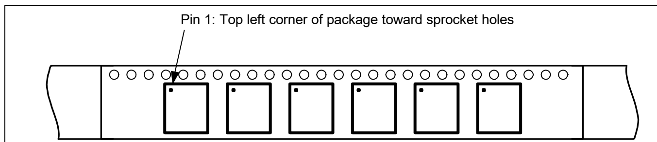
Figure 17 Pin 1 orientation
