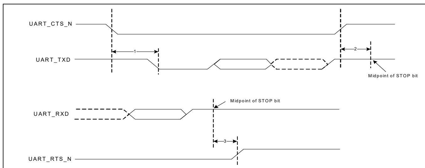
Figure 8 UART timing
