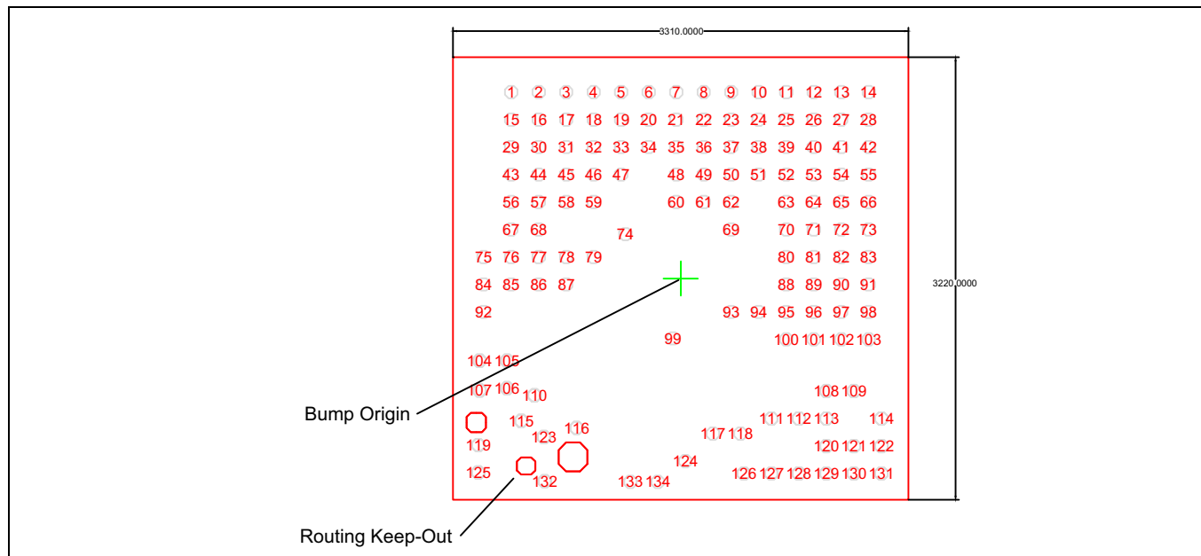
Figure 16 CYW20721YB2 WLCSP keep-out model
