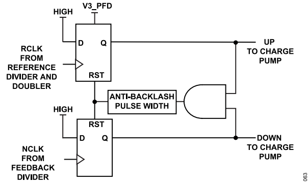
Figure 69. Simplified PFD Schematic
