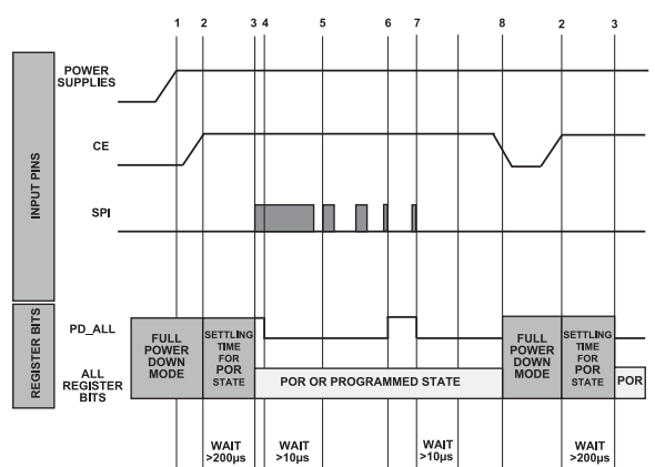
Figure 98. Power-Up and Initialization Sequence
