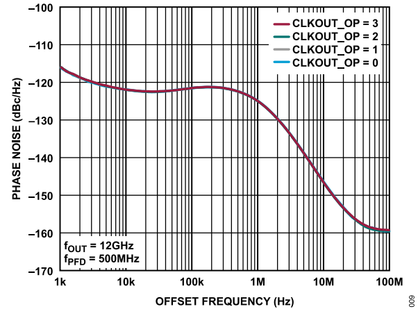
Figure 9. Closed-Loop Phase Noise at Various Output Amplitudes
