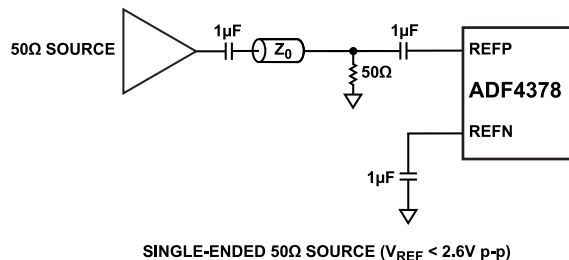
Figure 86. Single-Ended 50 \Omega Source ( V_{\text{REF}} < 2.6 \text{ V}_{\text{p-p}} )
