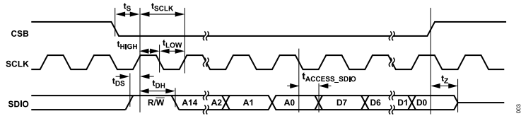
Figure 3. 3-Wire Read Timing Diagram (SDO_ACTIVE = 0)
