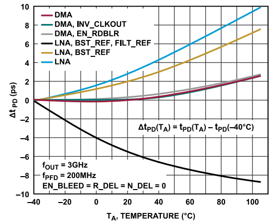
Figure 22. Delta Propagation Delay ( \Delta t_{PD} ) vs. T_A , Temperature, Device Configuration
