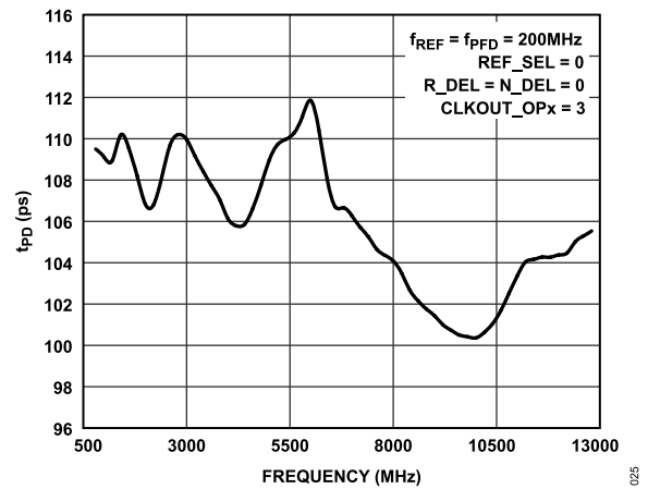
Figure 27. t_{PD} vs. Frequency
