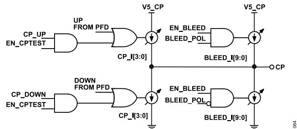
Figure 70. Simplified Charge-Pump Schematic
