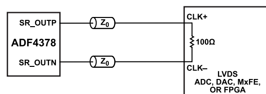
Figure 112. Common SYSREF Connections
