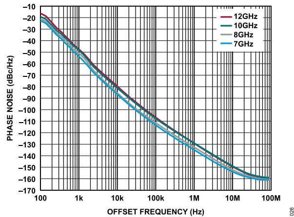
Figure 28. Open-Loop VCO Phase Noise at Various Frequencies
