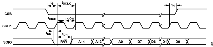
Figure 2. Write Timing Diagram
