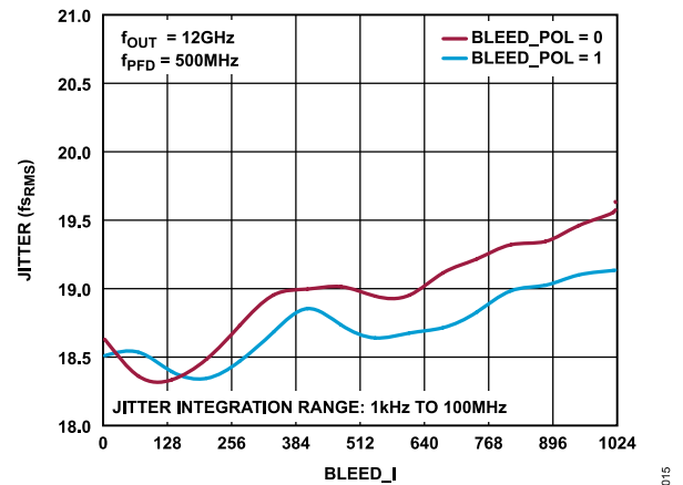
Figure 15. Jitter vs. BLEED\_I
