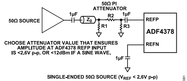
Figure 87. Single-Ended 50 \Omega Source ( V_{\text{REF}} > 2.6 \text{ V}_{\text{p-p}} )
