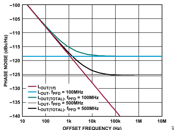
Figure 97. Theoretical In-Band Phase Noise, f_{OUT} = 10 GHz
