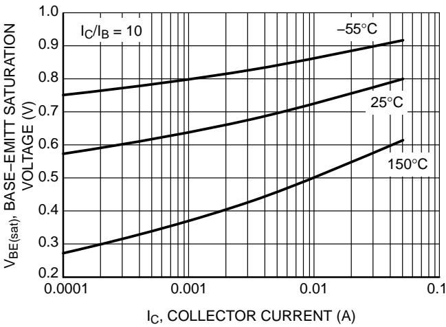
Figure 3. V_{BE(sat)} Curve
