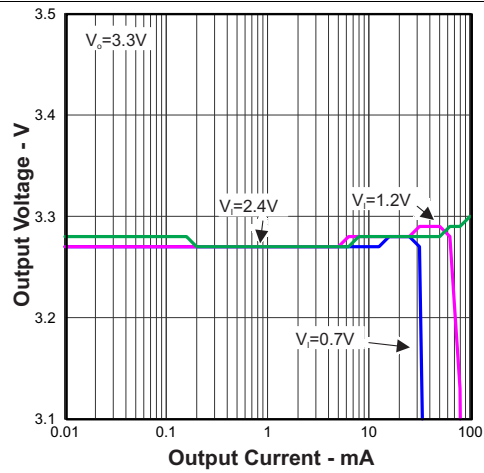
Figure 11. Output Voltage vs Output Current and Input Voltage
