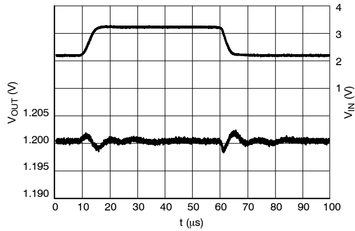
Figure 27. Line Transients, 1.2 V Version, t_R = t_F = 5 \mu\text{s} , I_{OUT} = 30 \text{ mA}
