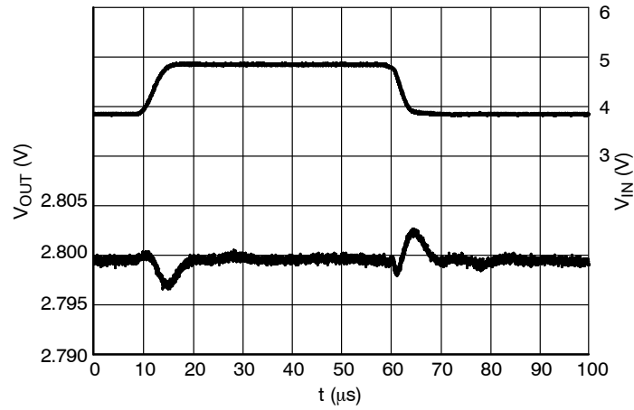
Figure 28. Line Transients, 2.8 V Version, t_R = t_F = 5 \mu\text{s} , I_{OUT} = 30 \text{ mA}
