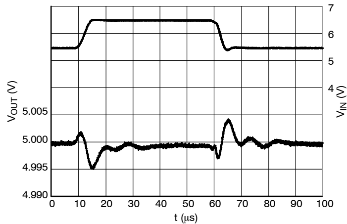
Figure 29. Line Transients, 5.0 V Version, t_R = t_F = 5 \mu\text{s} , I_{OUT} = 30 \text{ mA}
