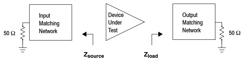
Figure 32. Series Equivalent Source and Load Impedance — 144 MHz
