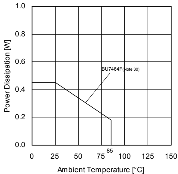
(g) BU7464F
