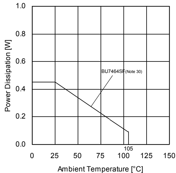
(h) BU7464SF
