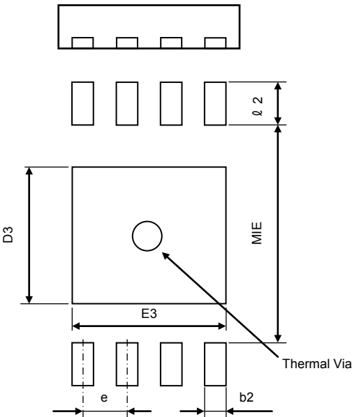
VSON008X2030
