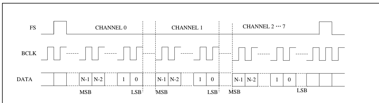
Figure 27 PCM Time Slot Audio Data
