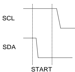
Figure 14 Valid START Condition
