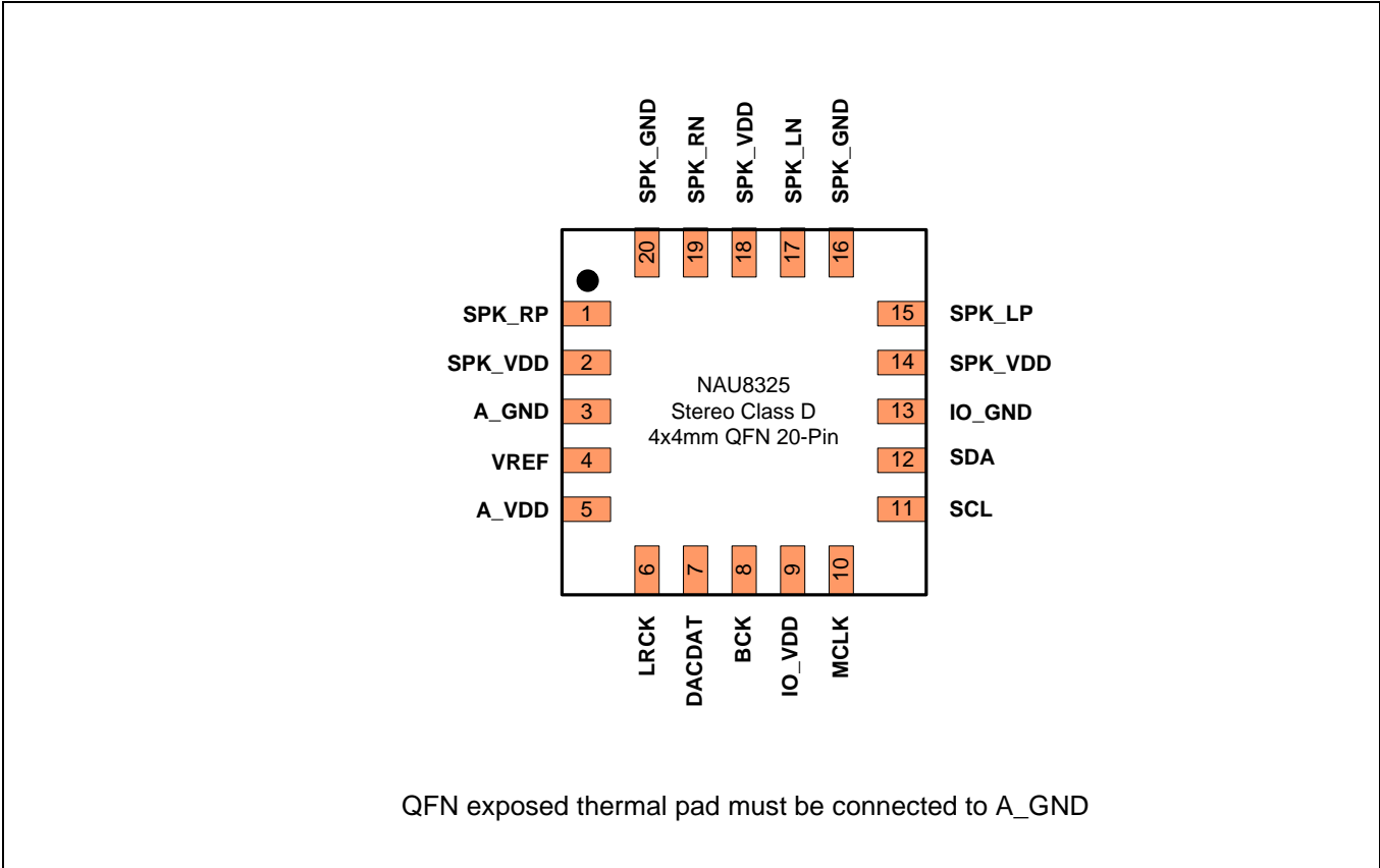
Figure 1 Pin Configuration of NAU8325 (TOP VIEW)
