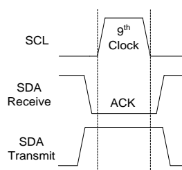
Figure 15 Valid Acknowledge
