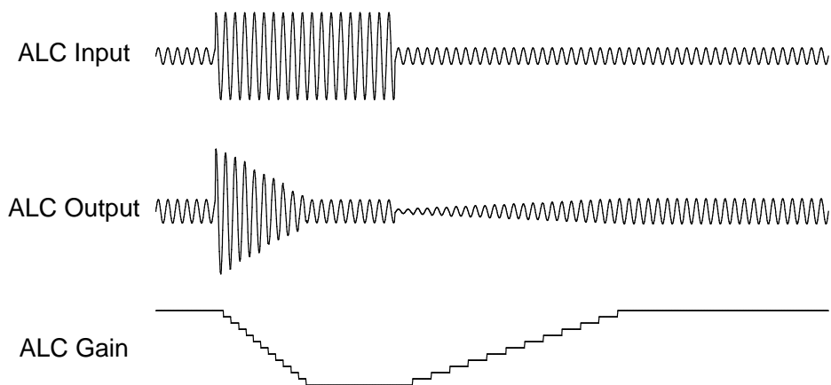
Figure 8 ALC Operation
