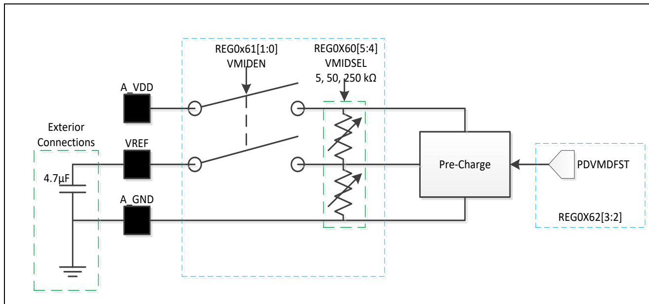
Figure 4 VREF Circuitry
