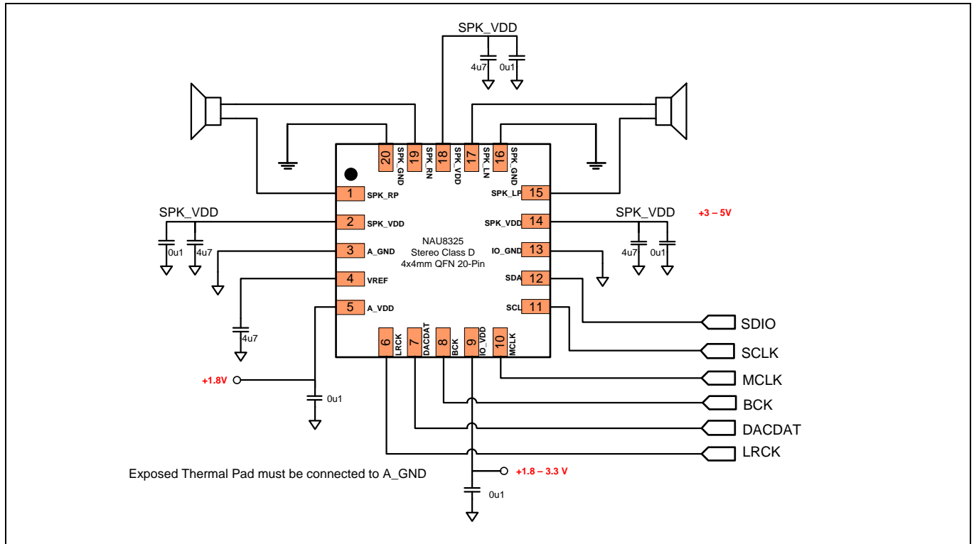
Figure 2 NAU8325 Simplified System Diagram
