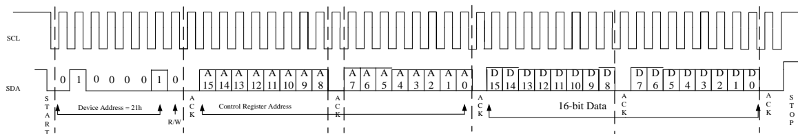
Figure 18 2-Wire Write Sequence
