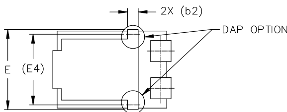
BOTTOM VIEW - DAP OPTION
