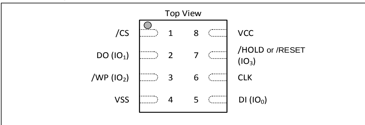
Figure 1b. W25Q32RV Pad Assignments, 8-pad WSON 6x5-mm, XSON 2x3-mm (Package Code ZP, XH)
