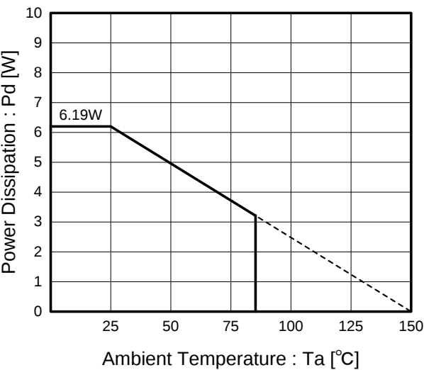
Figure 66. Thermal Reduction Characteristics
