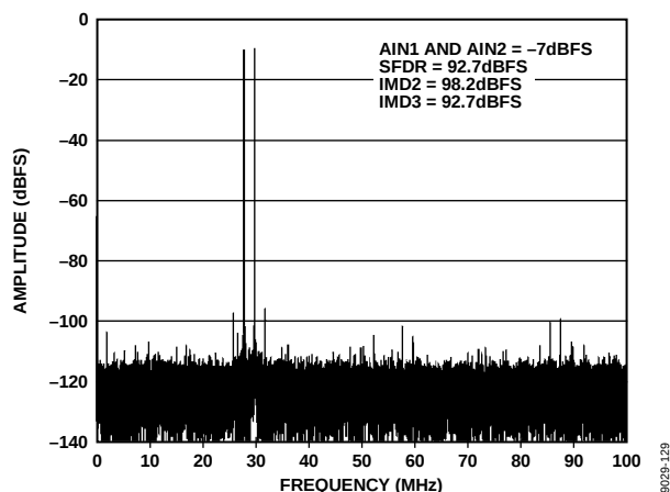
Figure 29. Two-Tone FFT with f_{IN1} = 170 MHz and f_{IN2} = 172 MHz, 2.5 V p-p FS, AD9467-200
