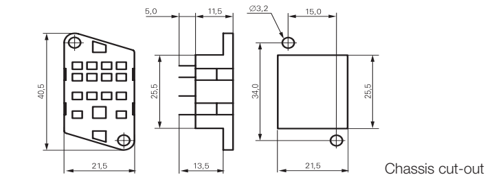
Chassis cut-out
