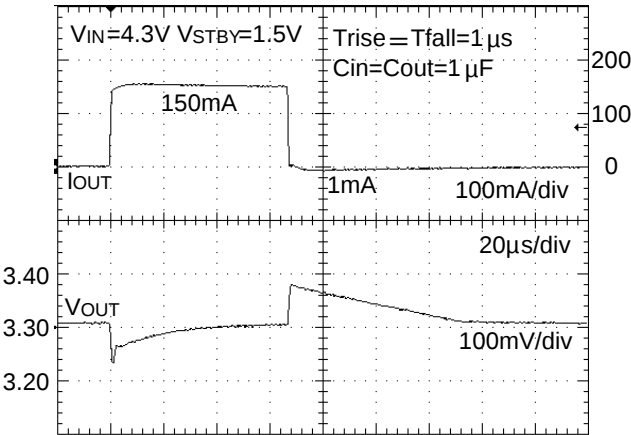
Figure 42. Load Response (1 to 150mA)
