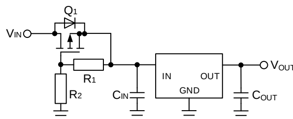
Figure 61. Protection against Reverse Polarity 3
