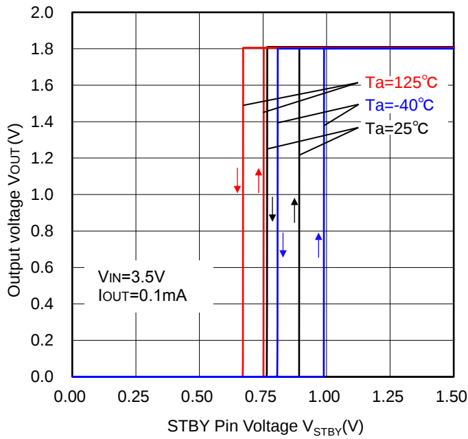
Figure 11. STBY Threshold
