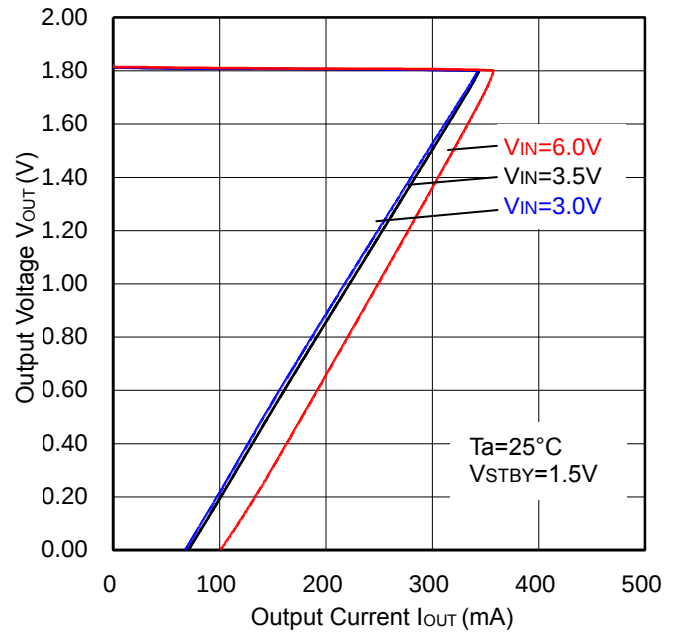
Figure 8. OCP Threshold
