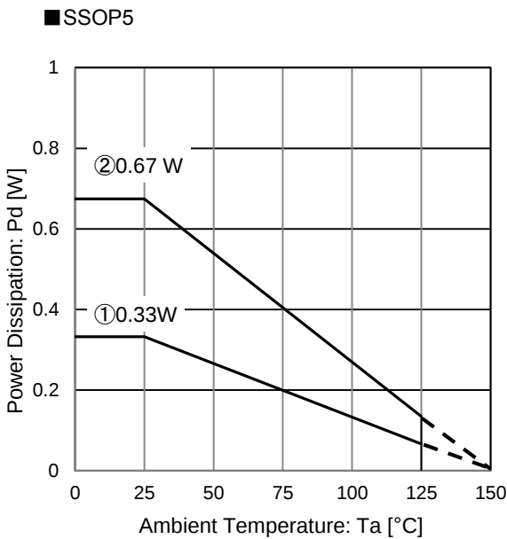
Figure 51. SSOP5 Package Data (Reference Data)
