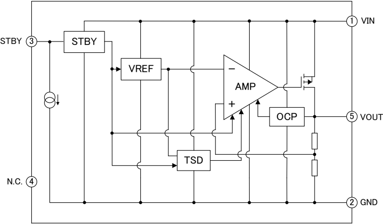
Figure 2. Block diagram
