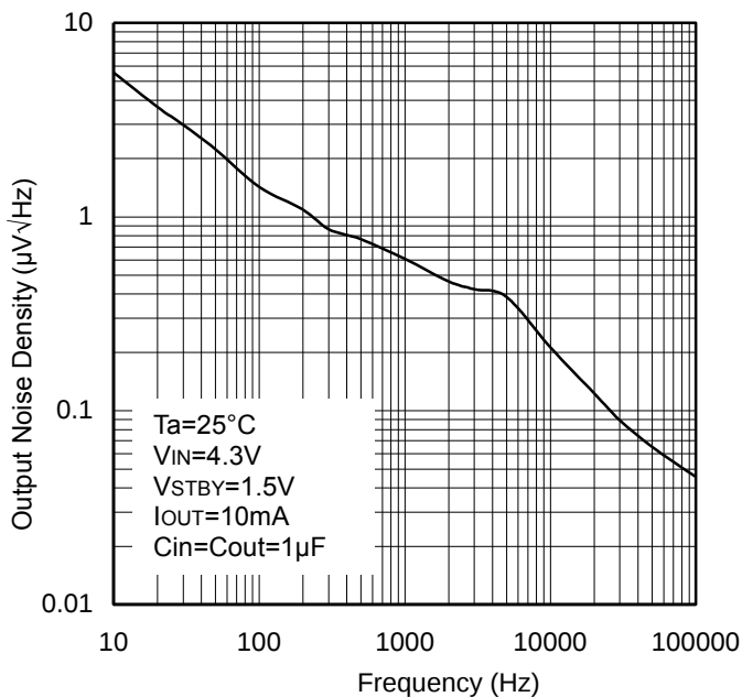
Figure 40. Output Noise Density vs Frequency
