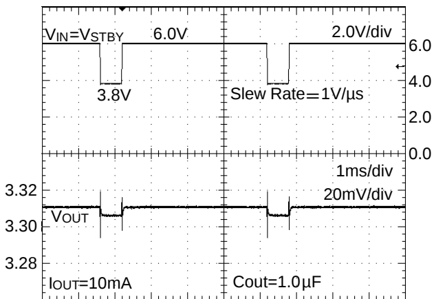
Figure 44. Line Transient Response (3.8 to 6.0V)
