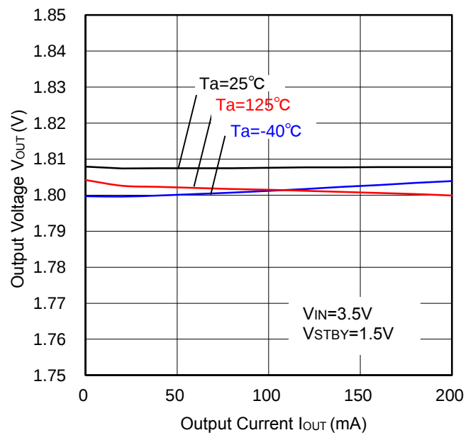
Figure 6. Load Regulation
