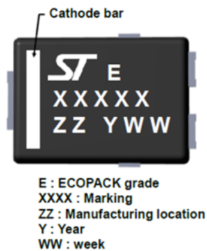
Figure 10. PSMC (TO-277A) marking
