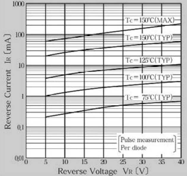
Reverse Current
