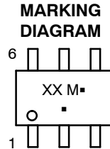
SOT-363/SC-88/ SC70-6 CASE 419B
