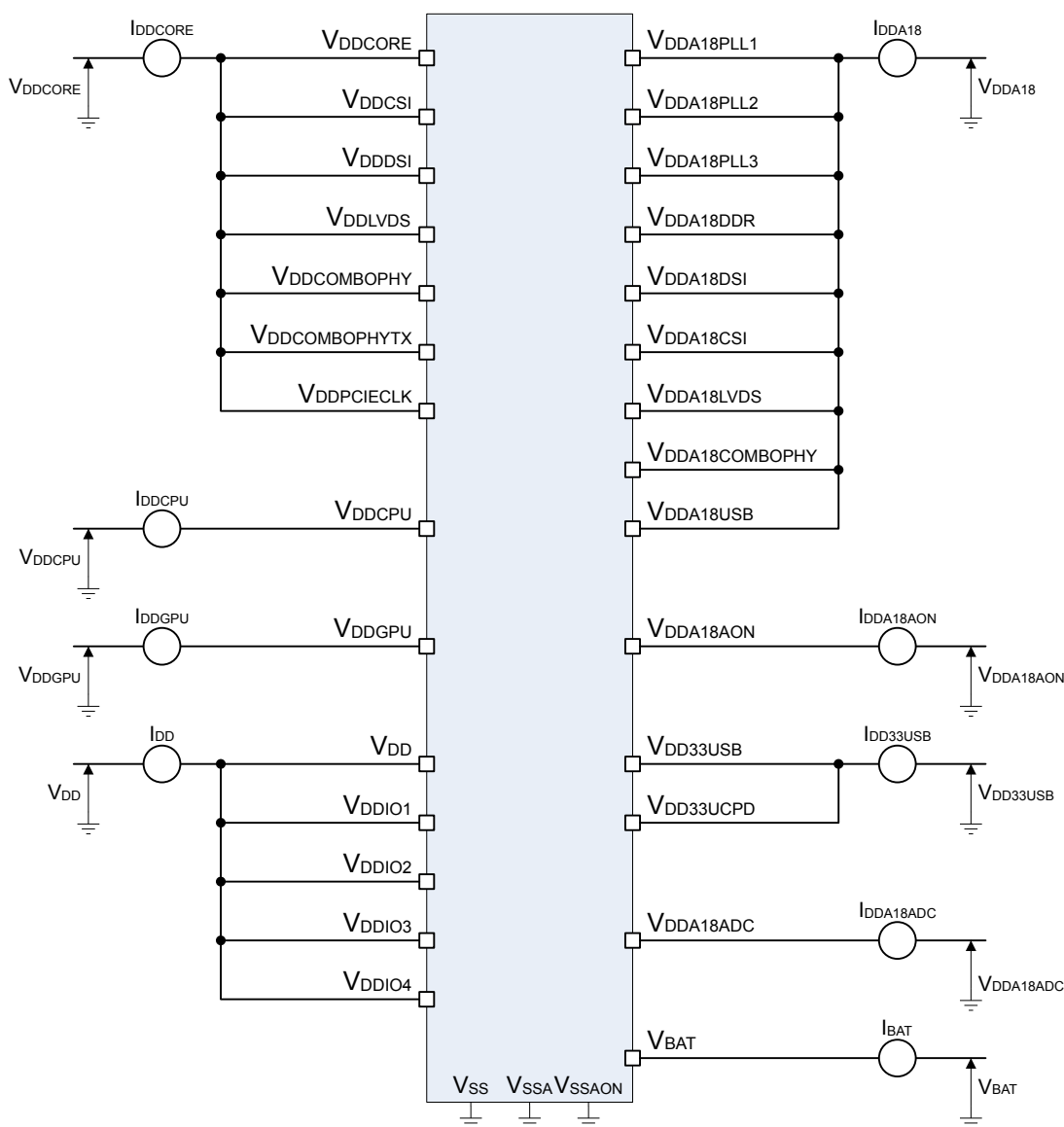
Figure 13. Current consumption measurement scheme
