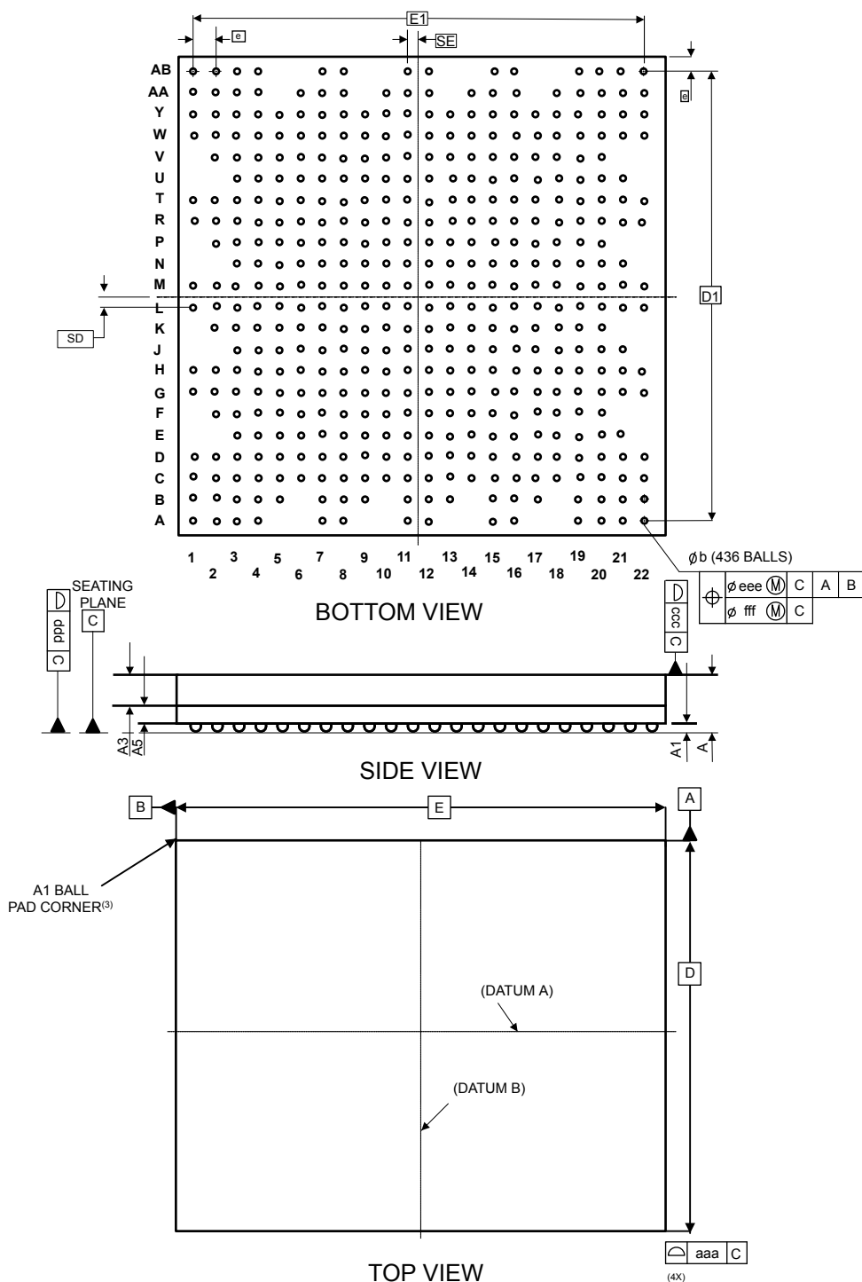
Figure 70. TFBGA436 - Outline
