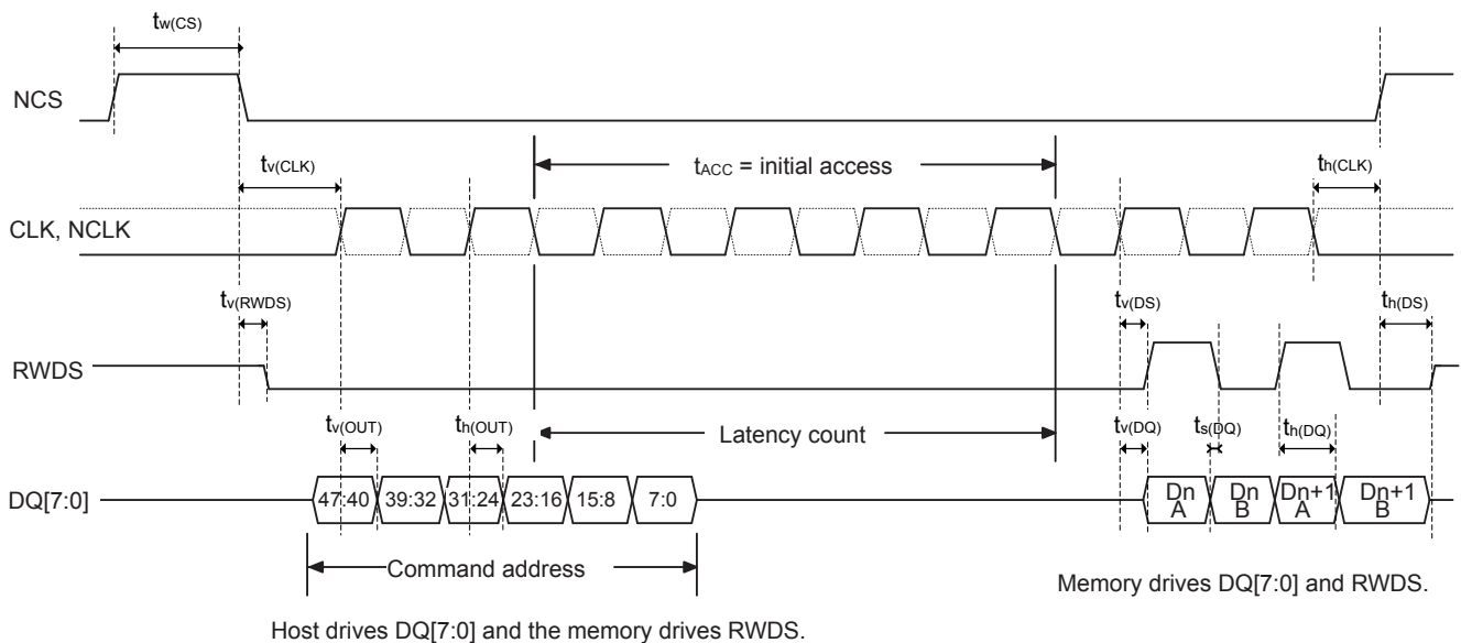
Figure 35. OCTOSPI HyperBus read
