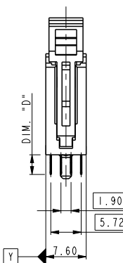
DETAIL A SCALE 3.000
