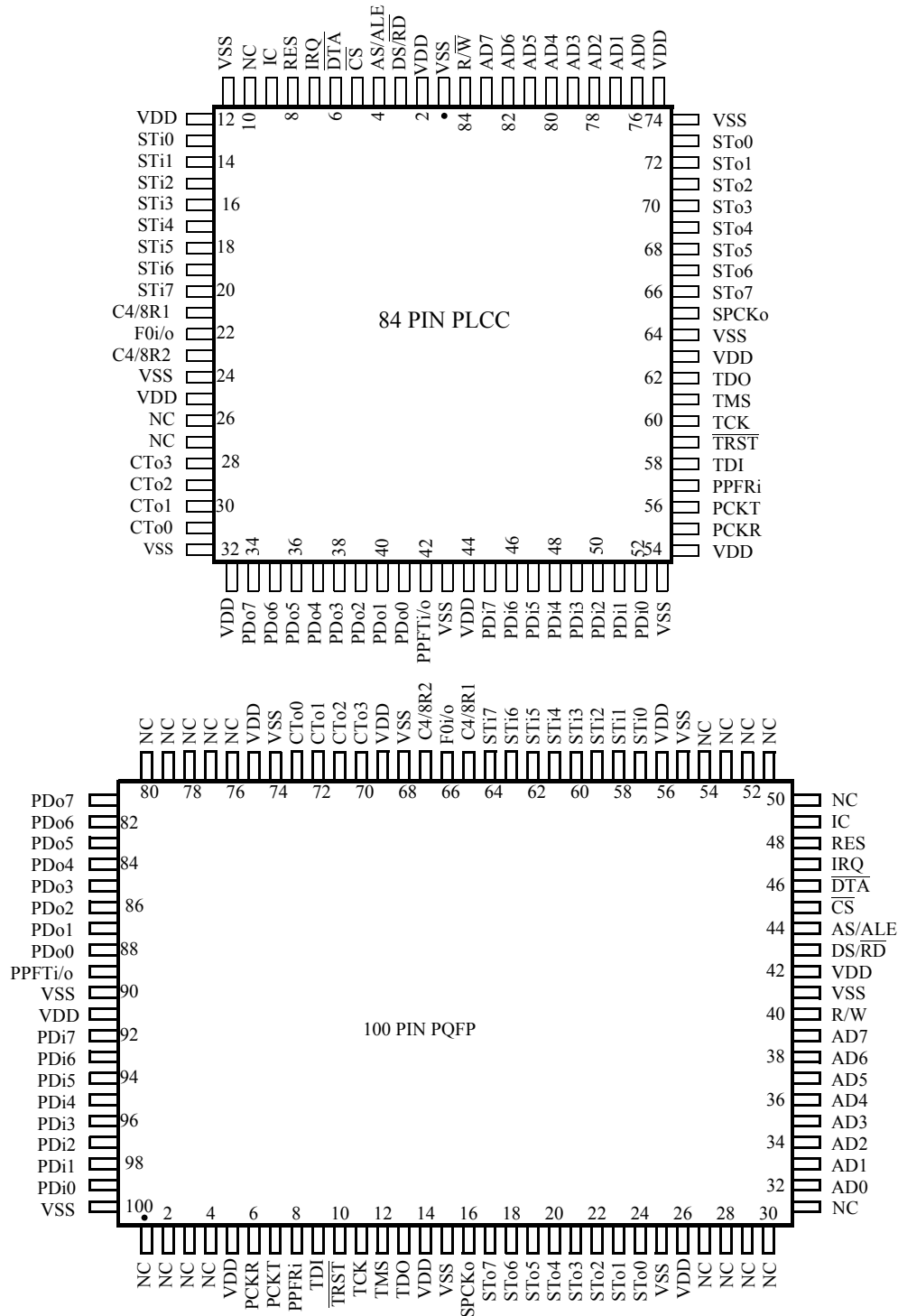
Figure 2 - Pin Connections
