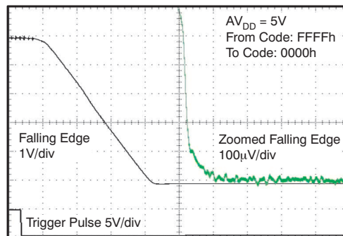
Figure 28. Full-Scale Settling Time 5-V Falling Edge
