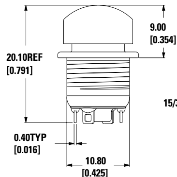
ACROSS FLATS
