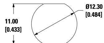
PANEL CUTOUT
