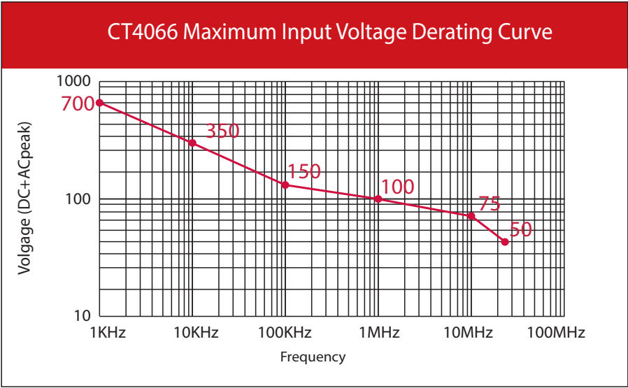
Figure 1 Derating Curve
