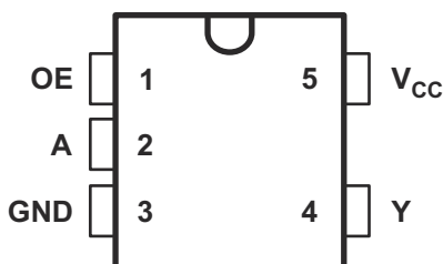
Figure 6-1. DCK or DBV Package, 5-Pin SC70 or SOT-23 (Top View)
