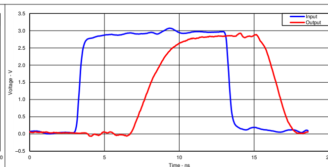
Figure 7-2. Switching Characteristics at 50 MHz Excellent Signal Integrity (3.3 V to 3.3 V at 3.3-V V_{CC} )
