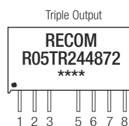
Pin Connections
