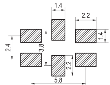
Figure 2) Land Pattern
