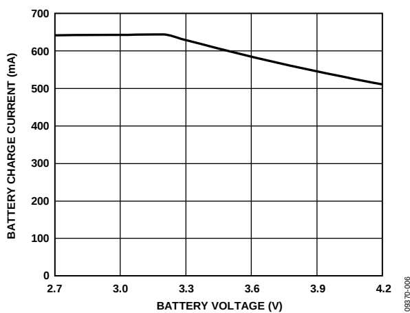
Figure 6. USB Compliant Charge Current vs. Battery Voltage, V_{IN} = 5.0\text{ V} , ILIM = 500\text{ mA}
