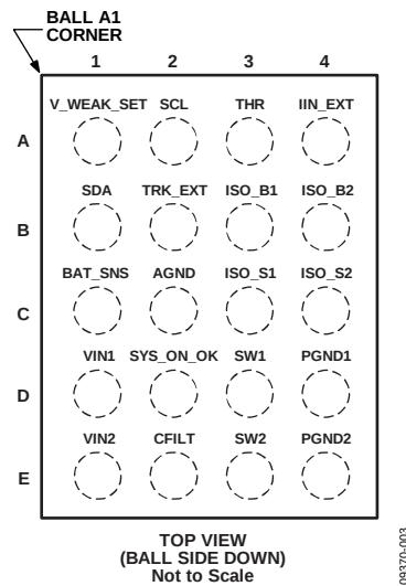
Figure 3. Pin Configuration
