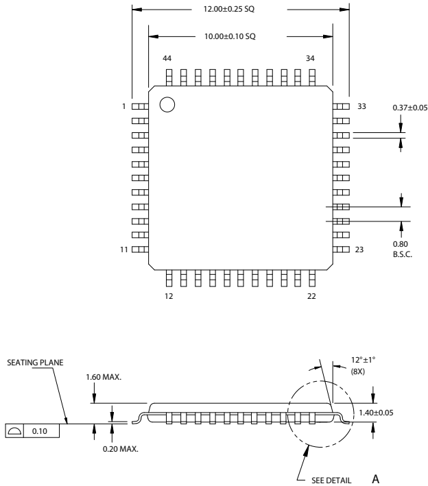
Figure 11. 44-Pin Thin Plastic Quad Flat Pack A44
