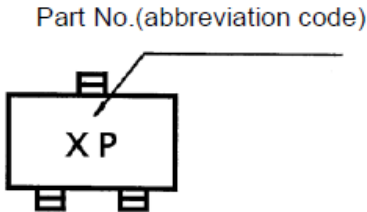
Fig. 8.2 Marking RN1313
