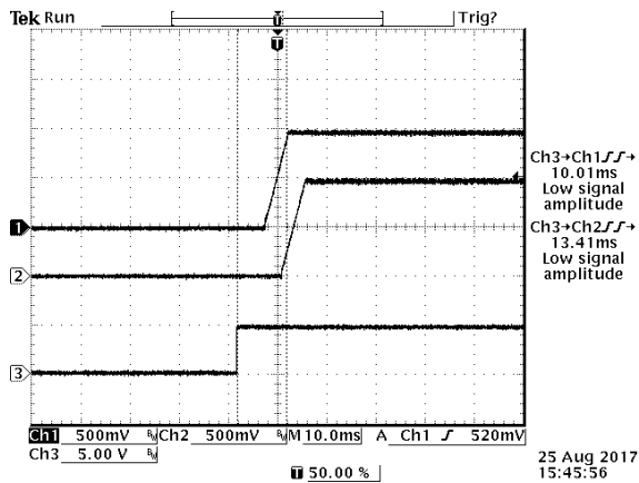
Figure 39. Startup from EN Ch1: V_{out1} ; Ch2: V_{out2} ; Ch3: EN (EN1&EN2) Test Condition: V_{out1}=1.0V/40A ; V_{out2}=1.0V/40A at V_{in}=11V@T_a=25^{\circ}C
