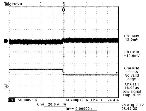
Figure 16. V_{in}=11V , V_o=1.0V , I_o=75\%-50\%I_o \text{ max} , di/dt=1A/us
