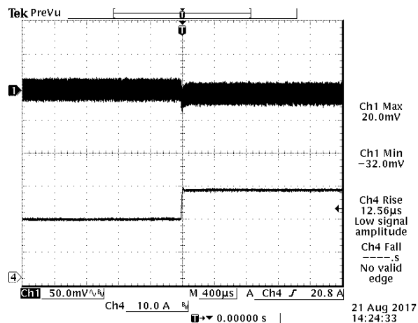
Figure 17. V_{in}=11V , V_o=1.8V , I_o=50\%-75\%I_o \text{ max} , di/dt=1A/us
