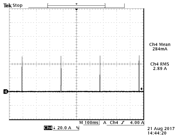
Figure 26. Vout2 Output current @ SCP, V_{in} = 11V , V_{out} = 1.8V , T_a = 25^\circ C
