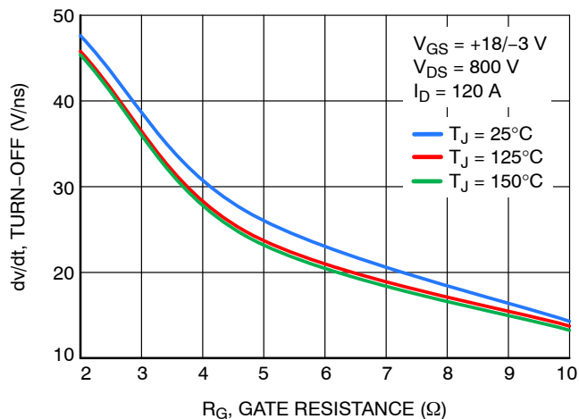
Figure 24. \frac{dv}{dt} Turn OFF vs. Gate Resistance V_{DS} = 800\text{ V}
