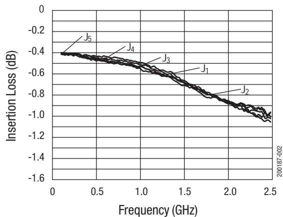
Figure 2. Typical Loss (All Paths) vs Frequency
