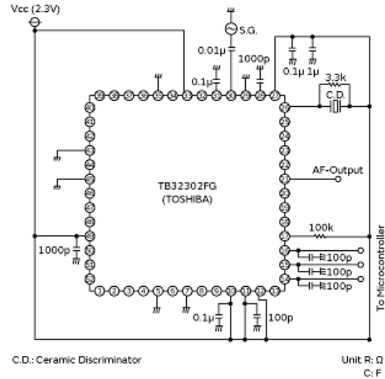
Measurement Circuit
