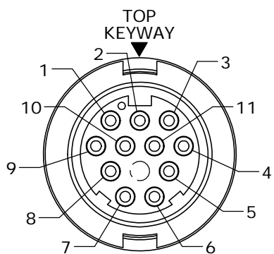
FACE VIEW W3282-11PG-3XX(W)
