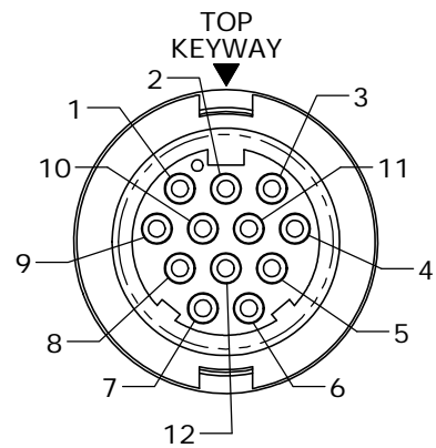
FACE VIEW W3282-12PG-3XX(W)
