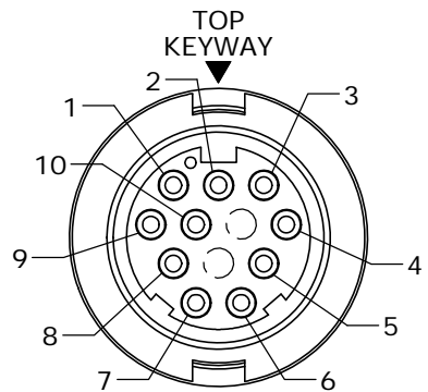
FACE VIEW W3282-12PG-3XX(W)
