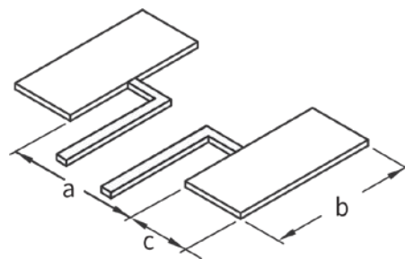
Solder Pad
