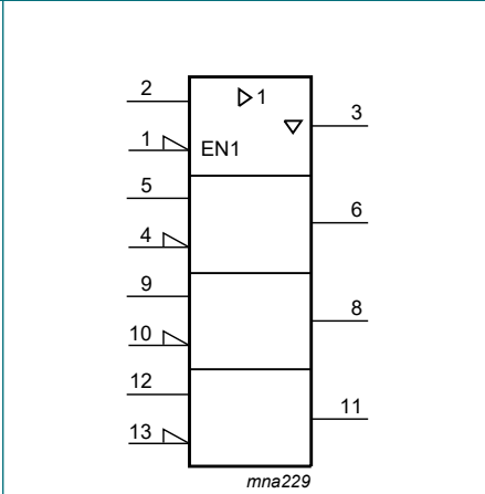
Fig. 2. IEC logic symbol
