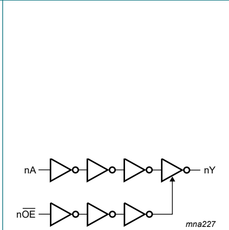
Fig. 3. Logic diagram
