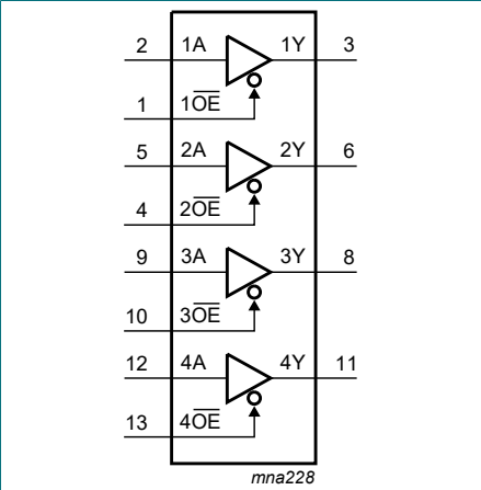
Fig. 1. Logic symbol
