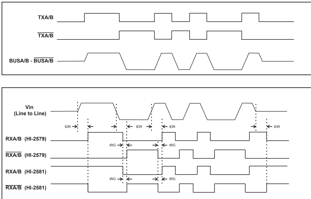
Figure 2. Example Waveforms
