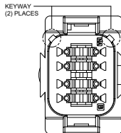
P/N AT04-08PB KEY-B CONFIGURATION STANDARD COLOR: BLACK
