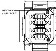
P/N AT04-08PD KEY-D CONFIGURATION STANDARD COLOR: BROWN
