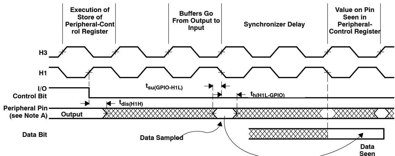
Figure 35. Change of Peripheral Pin From General-Purpose Output to Input Mode Timing
