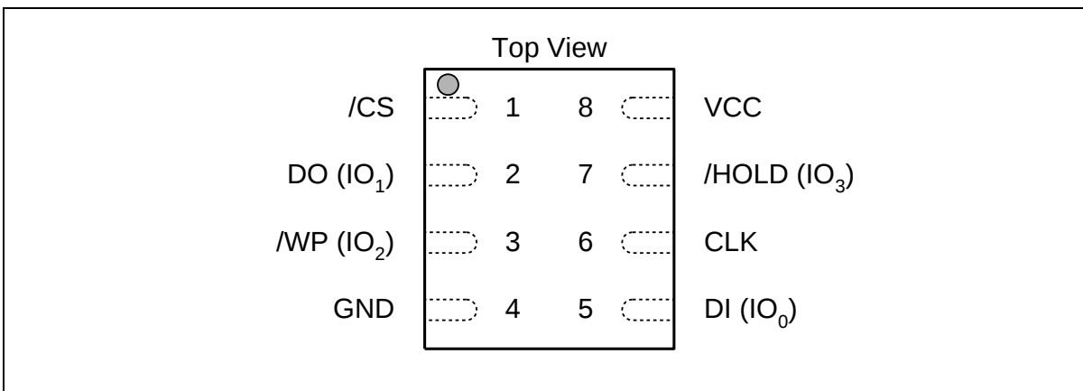
Figure 1. W25N01KV Pad Assignments, 8-pad WSON 6x5mm and 8x6-mm (Package Code ZP, ZE)
