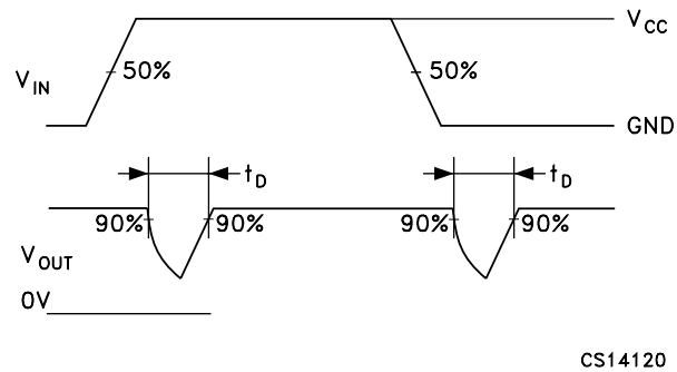
Figure 10. Switching time and charge injection ( V_{GEN} = 0\text{ V} , R_{GEN} = 0\text{ }\Omega , R_L = 1\text{ M}\Omega , C_L = 100\text{ pF} )
