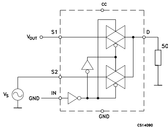
Figure 7. Test circuits
