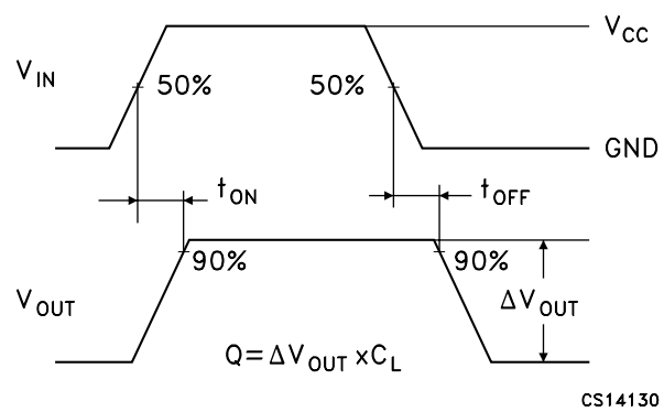
Figure 11. Switching time and charge injection ( V_{GEN} = 0\text{ V} , R_{GEN} = 0\text{ }\Omega , R_L = 1\text{ M}\Omega , C_L = 100\text{ pF} ) 2
