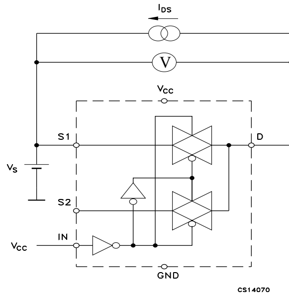
Figure 3. On-resistance
