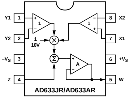
Figure 3. 8-Lead SOIC
