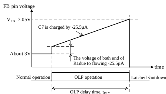
Figure 8-30. OLP Operation
