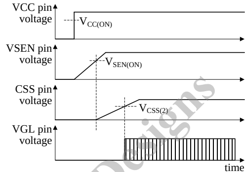
Figure 8-14. Startup Waveforms
