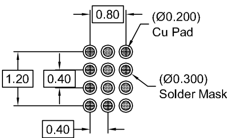
RECOMMENDED LAND PATTERN (NSMD PAD TYPE)
