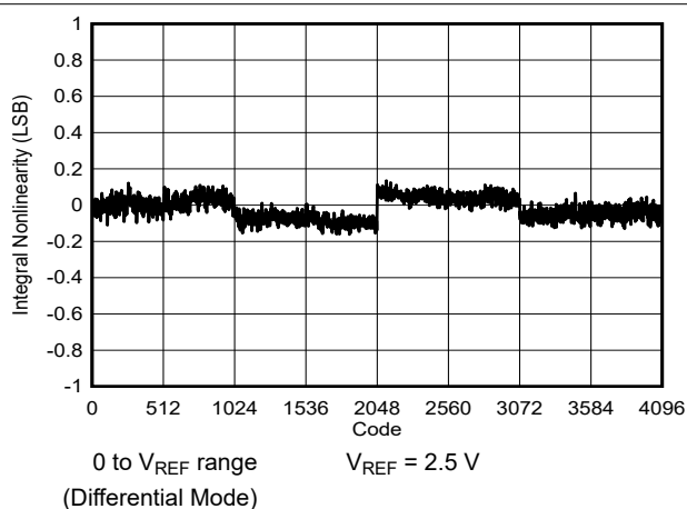
Figure 6-25. Integral Linearity Error vs Code
