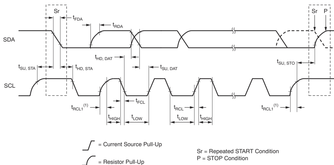
Figure 6-2. Timing for High-Speed (Hs) Mode Devices on I²C Bus
