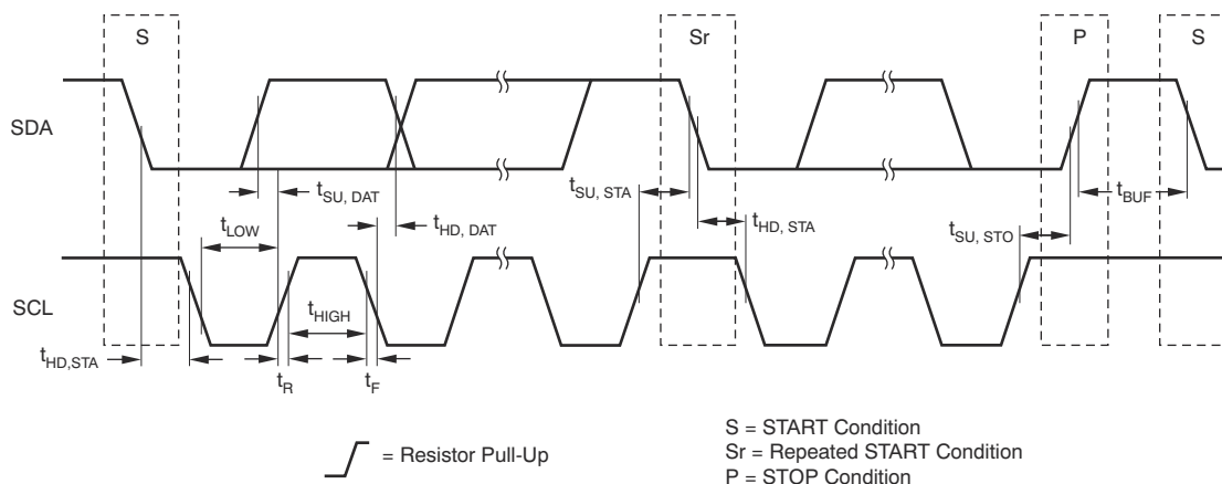
Figure 6-1. Timing for Standard and Fast Mode Devices on I²C Bus
